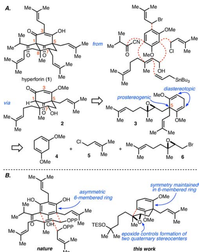
Scheme 1. (A) Synthesis Strategy for Hyperforin (1) and (B) Comparison of This Work to Hyperforin Biosynthesis
